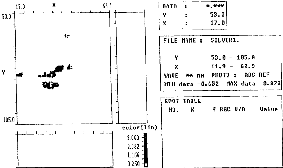
FIGURE 6. Dual wavelength background subtraction.
