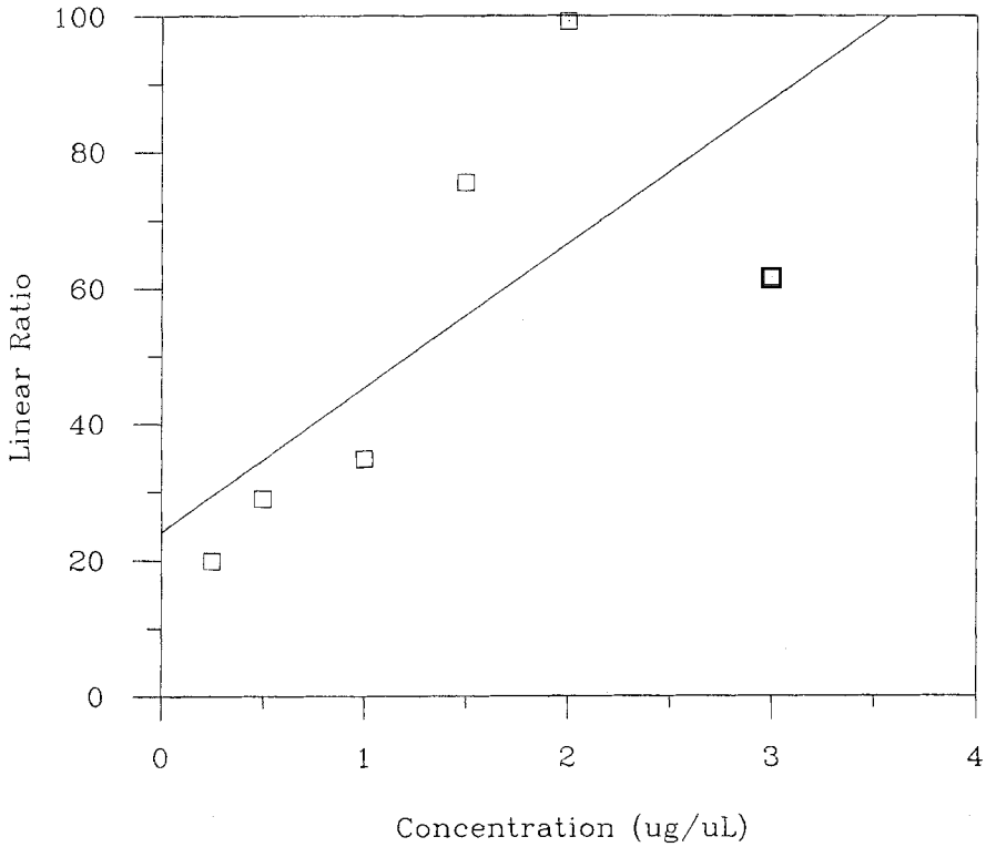
FIGURE 8. Calibration curve from raw volumes - Phosphatidyl Inositol.
